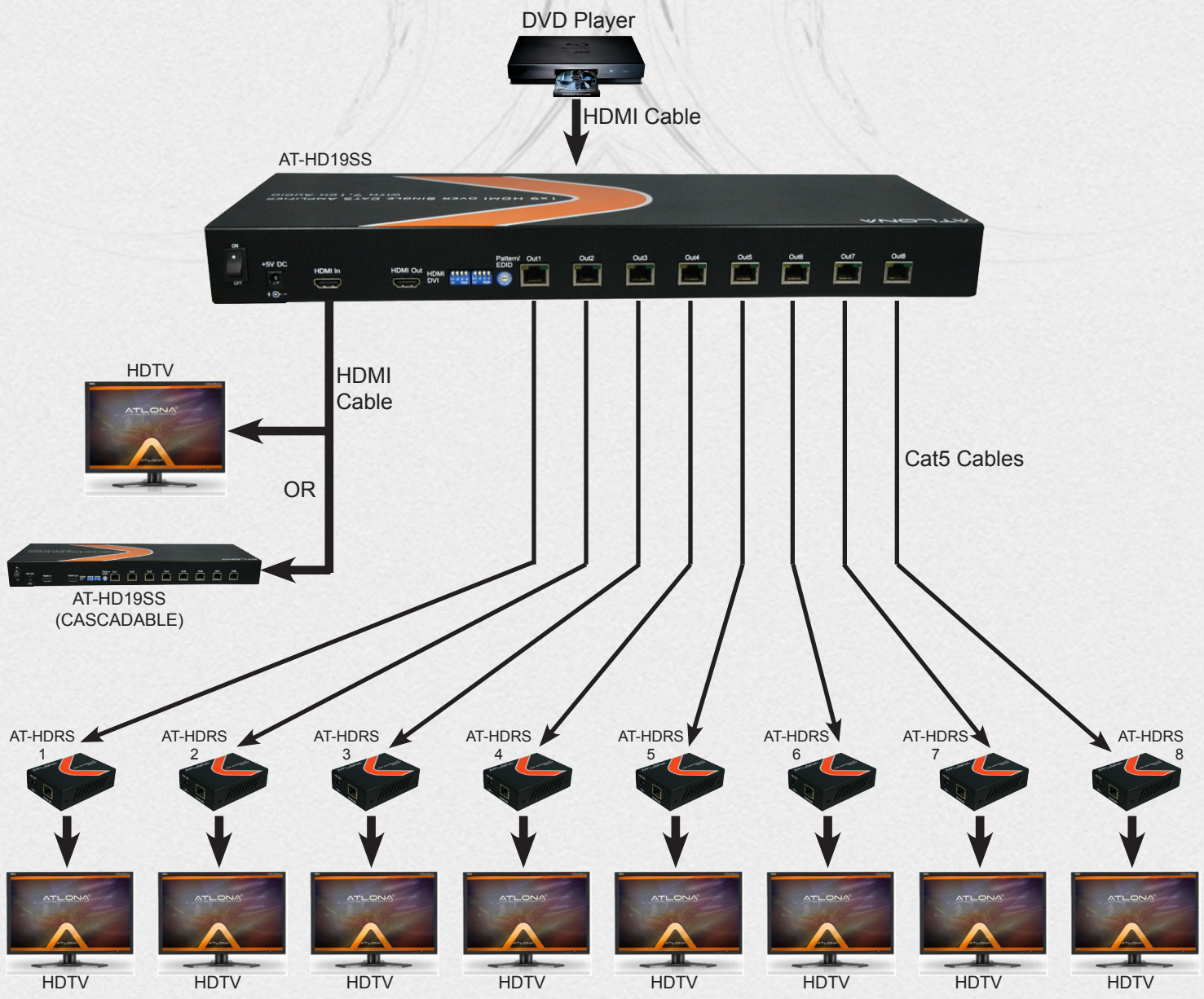
Connection Diagram
